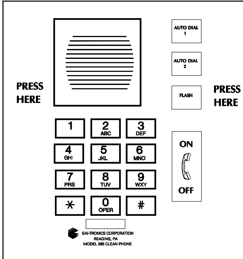
Figure 2. Front panel with pressure points shown
