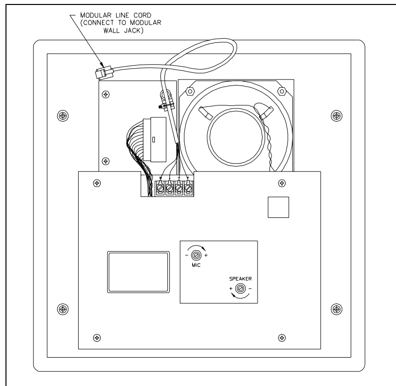
Figure 5. Microphone and Speaker Adjustments
